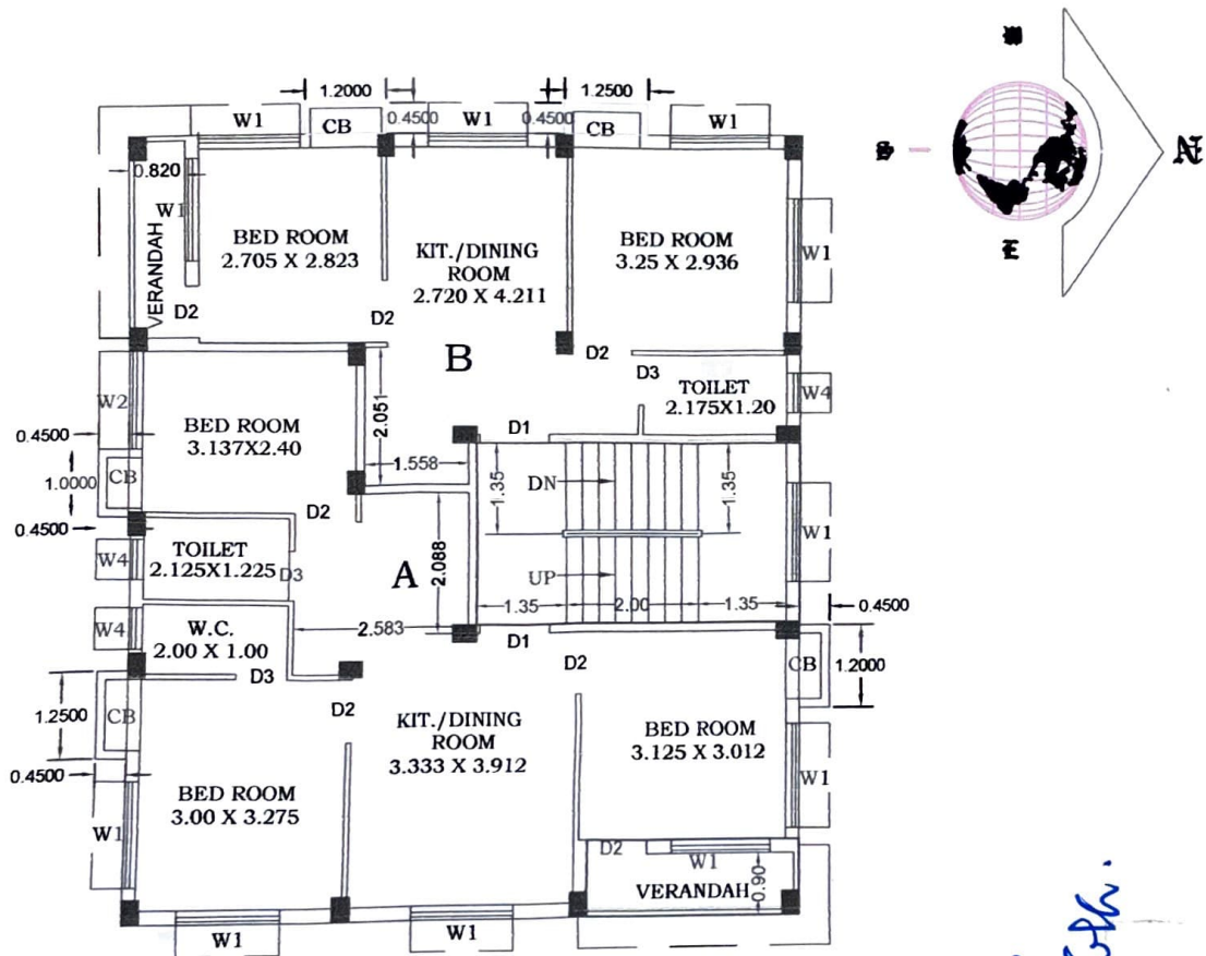
1ST & 2ND FLOOR PLAN SCALE:- 1:100
