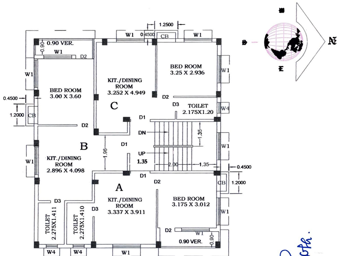
3RD FLOOR PLAN SCALE:- 1:100
